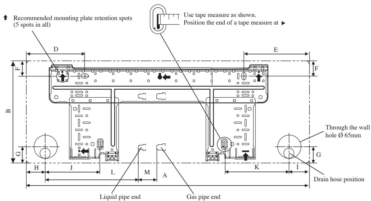
INSTALLATION PLATE FTXN25/35MV1B
